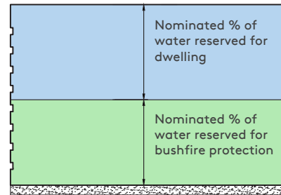
Typical Dual Purpose Bushfire Protection Tank
